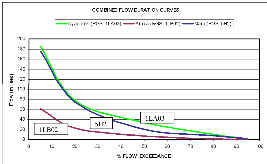
Figure 5.1. Combined flow duration curves 3 RGS on Mara River from 1955 to 2007.
