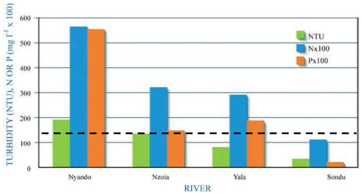
Figure 5.5. Comparison of turbidity, Nitrogen and Phosphorus rates in four major Kenyan rivers in the Lake Victoria Basin over three successive years (2000-2002).
