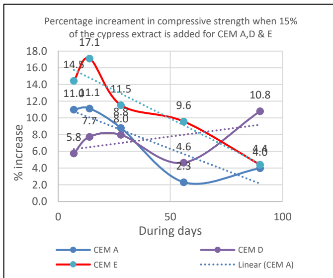
Fig 4. Percentage increasement on the compressive strength for CEM A, D and E when 15% of the cypress extract added from the control.
