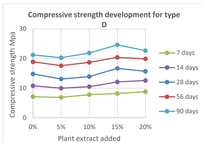
Fig 2. Effect of pant extract on the compressive strength at 28 days and 56 days using type D cement
