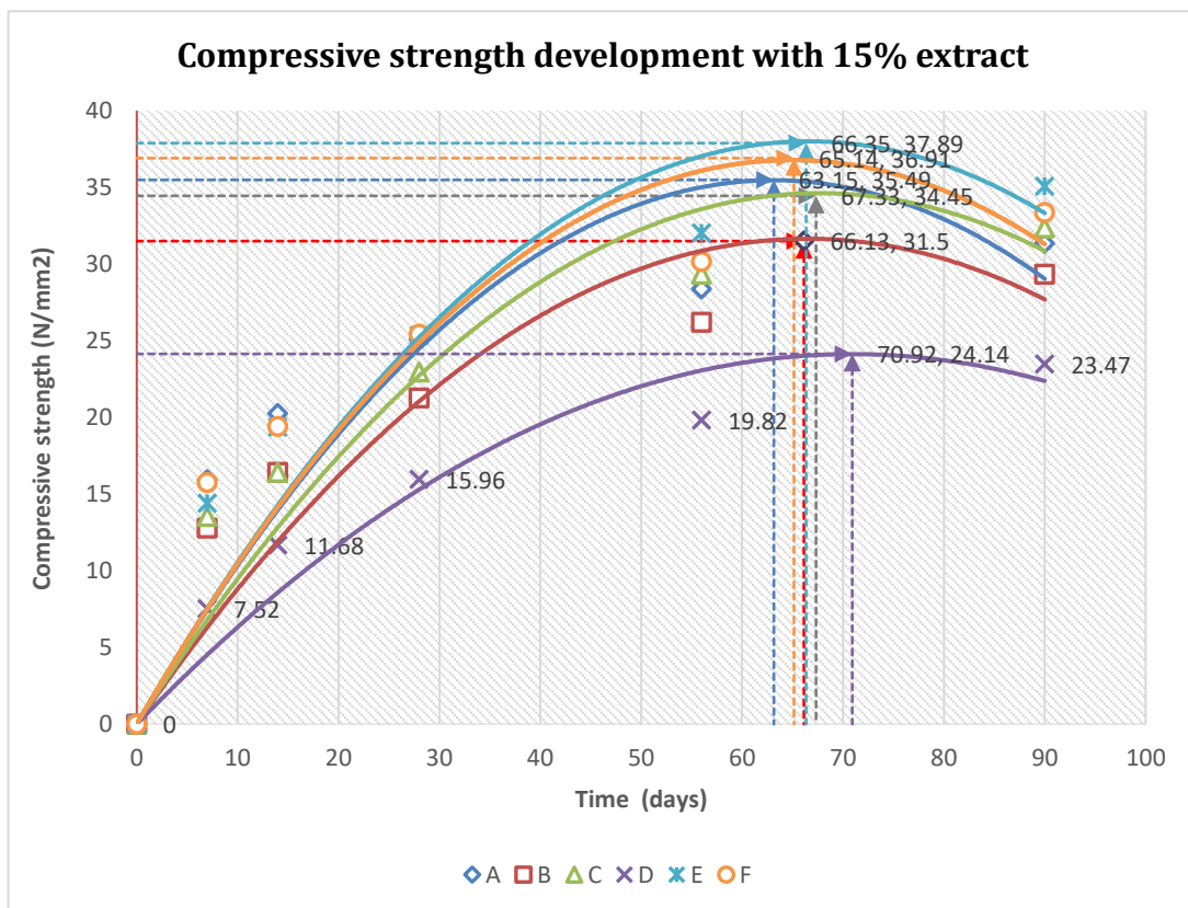
Fig. 5. Compressive strength development of the cement types when 15% of the cypress tree extract is added.
