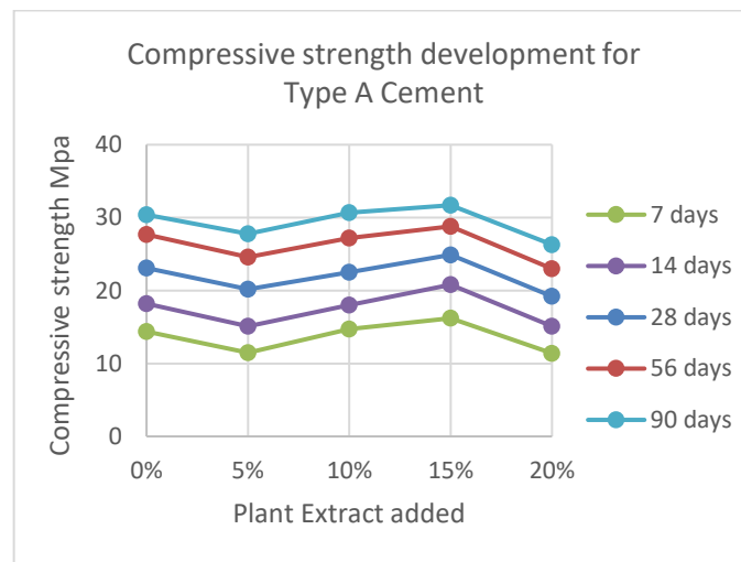
Fig 1. Effect of cypress tree extract on the compressive strength for cement type A
