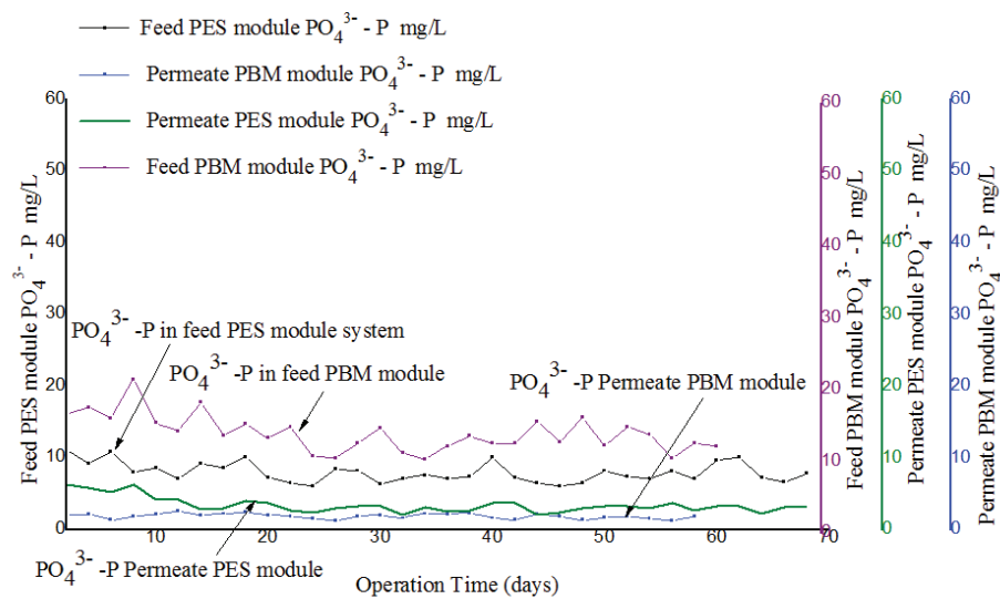
Figure 12: Comparison of phosphate (PO 4 3- -P) in feed and in permeate for experiment conducted with PES membrane module and PBM-coated membrane module.
