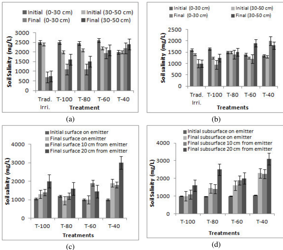
Figure 2. The effect of deficit irrigation on soil salinity: (a) and (b) are vertical salt distribution near emitter and at the depths of 0-30 and 30-50 cm for summer vs. winter seasons respectively, and (c) and (d) are horizontal salt distribution during the winter season for surface vs. subsurface soil samples
