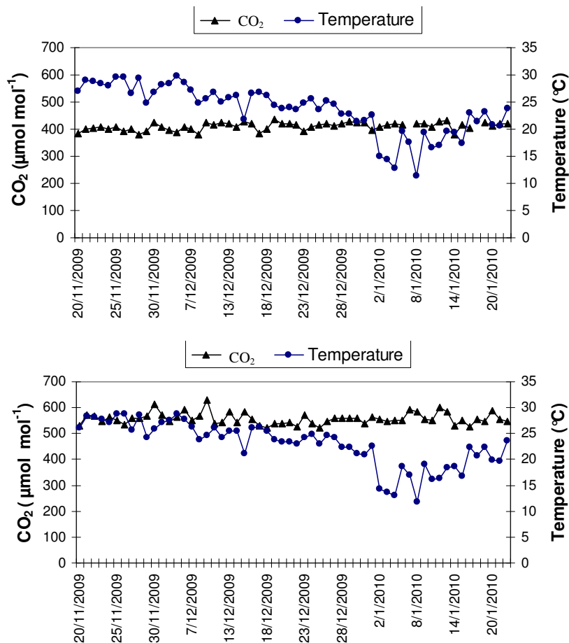
Figure 1. Level of CO 2 concentration and mean day temperature inside Open Top Chambers (OTCs) used for ambient (A) and high CO 2 exposure (B).
