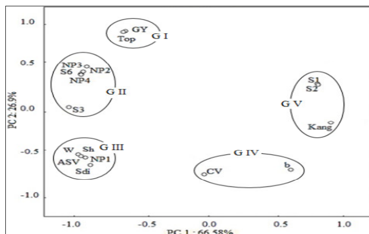
Figure 2. Biplot of PCA1 versus PCA2 for different parametric and non-parametric measures of stability. GY; W_i^2 ; \sigma_i^2 ; b_i ; CV_i ; S_{di}^2 ; ASV; S^{(1)} - S^{(6)} ; NP1 - NP4 ; R -sum, and Top indicate: Mean Grain Yield; Wricke's ecovalence; Shukla's stability variance; regression coefficient of Eberhart and Russell; Francis and Kannenberg's Coefficient of Variability; deviation from regression (Eberhart and Russell); AMMI Stability Value of Purchase et al. ; Nassar and Huehn's non-parametric stability statistics; Thennarasu's Non-Parametric stability statistics; Kang's rank-sum, and Fox-rank, respectively.
