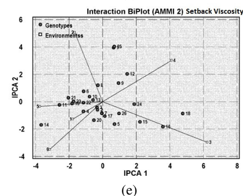
Figure 3. Interaction Biplot (AMMI II) for: (a) peak viscosity, Trough Viscosity, (c) Breakdown Viscosity, (d) Final Viscosity and (e) Setback Viscosity. Interaction BIPLLOT (AMMI II) for starch pasting characteristics across environments. the genotypes are labelled as 1-DL880,2-DL882,3-DL886,4-DL892,5-DL893,6-DL898,7-DL899,8-DL901,9-DL902,10-DL903,11-DL908,12-DL910,13-DL919,14-DL924,15-DL927,16-DL935,17-DL940,18-DL954,19-DL966,20-DL960,21-DL974,22-DL976,23-DL973,24-PBW343, 25-HD2329 and 26-RAJ3765.
