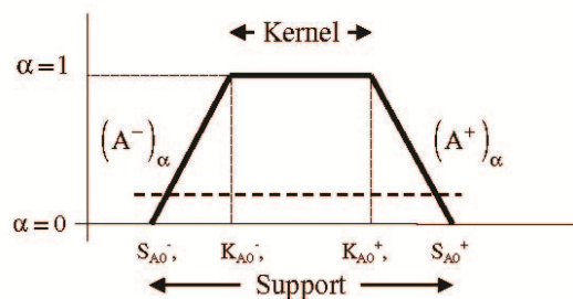
Figure 1. Fuzzy trapezoidal number.
