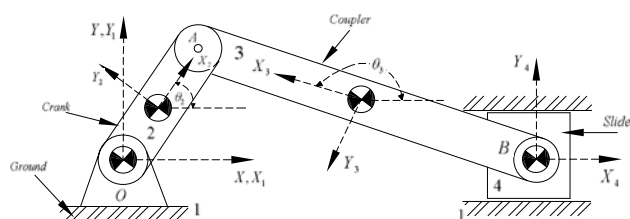
Fig. 4. Slider-crank mechanism
