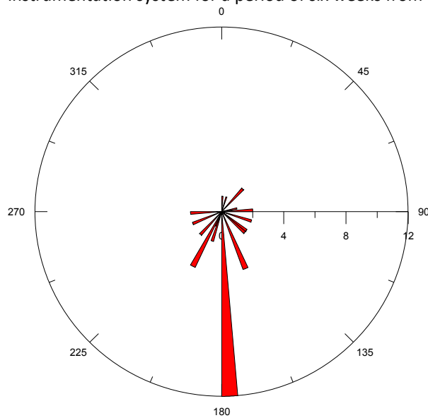
Figure 4: Wind rose for 2 m height at 9.00 a.m in Juja
