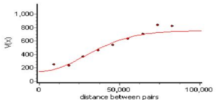
Figure 3 Best Fitting Gaussian Variogram for the three years mean rainfall data for all the fifty-three station in the whole Nzoia river Basin.
