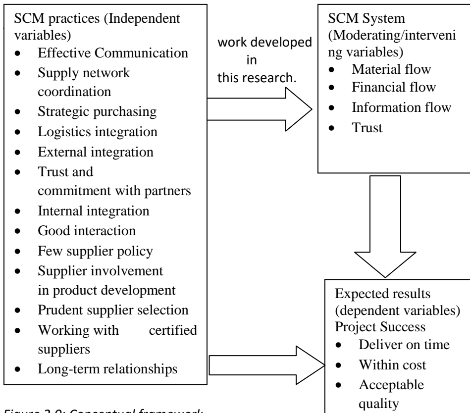
Figure 2.0: Conceptual framework
