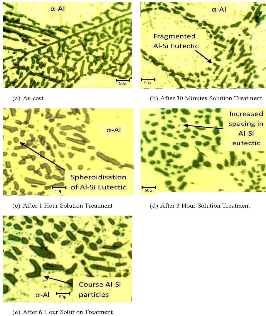
Fig. 4. Microstructures for the section with the cooling rate of 1.14^{\circ}\text{C/s} (a) in the as cast state (b) after solution treatment of 30 minutes (c) 1 hour and (d) 3 hours and (e) 6 hour sat 540^{\circ}\text{C} .
